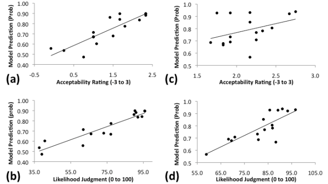
Figure 1: (a) Model fits against Cummins' AC acceptability ratings. (b) Model fits against diagnostic likelihood judgments. (c) Model fits against Cummins' MP acceptability ratings. (d) Model fits against predictive likelihood judgments.
